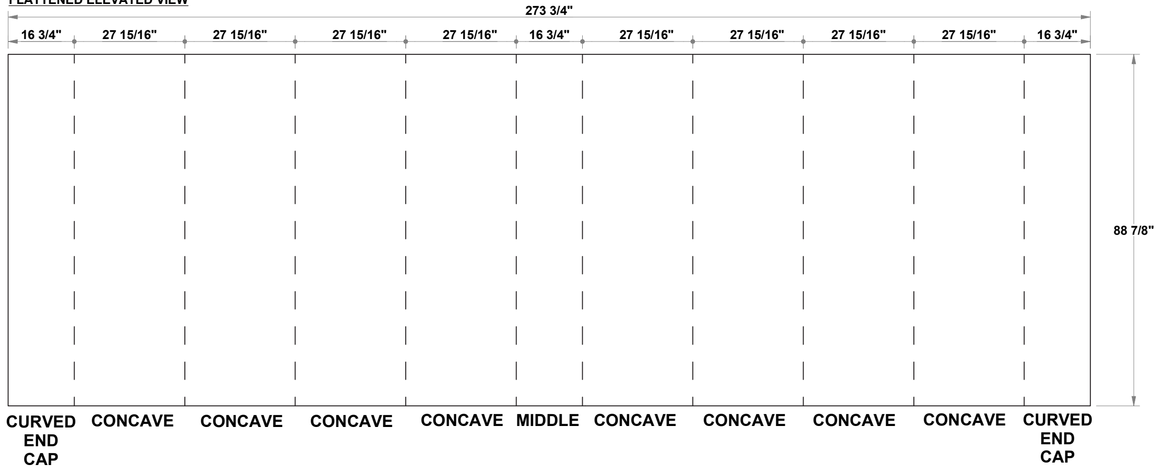
FLATTENED ELEVATED VIEW
