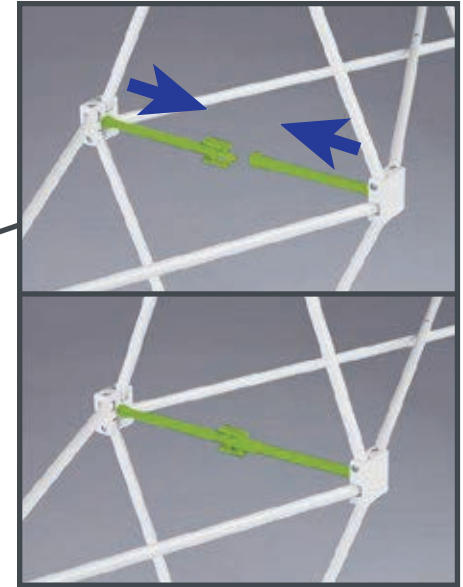
INTERNAL FRAME LOCKS
