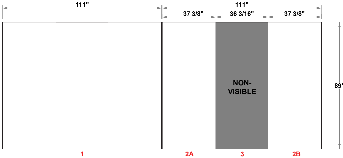
MURAL FLATTENED ELEVATED VIEW
