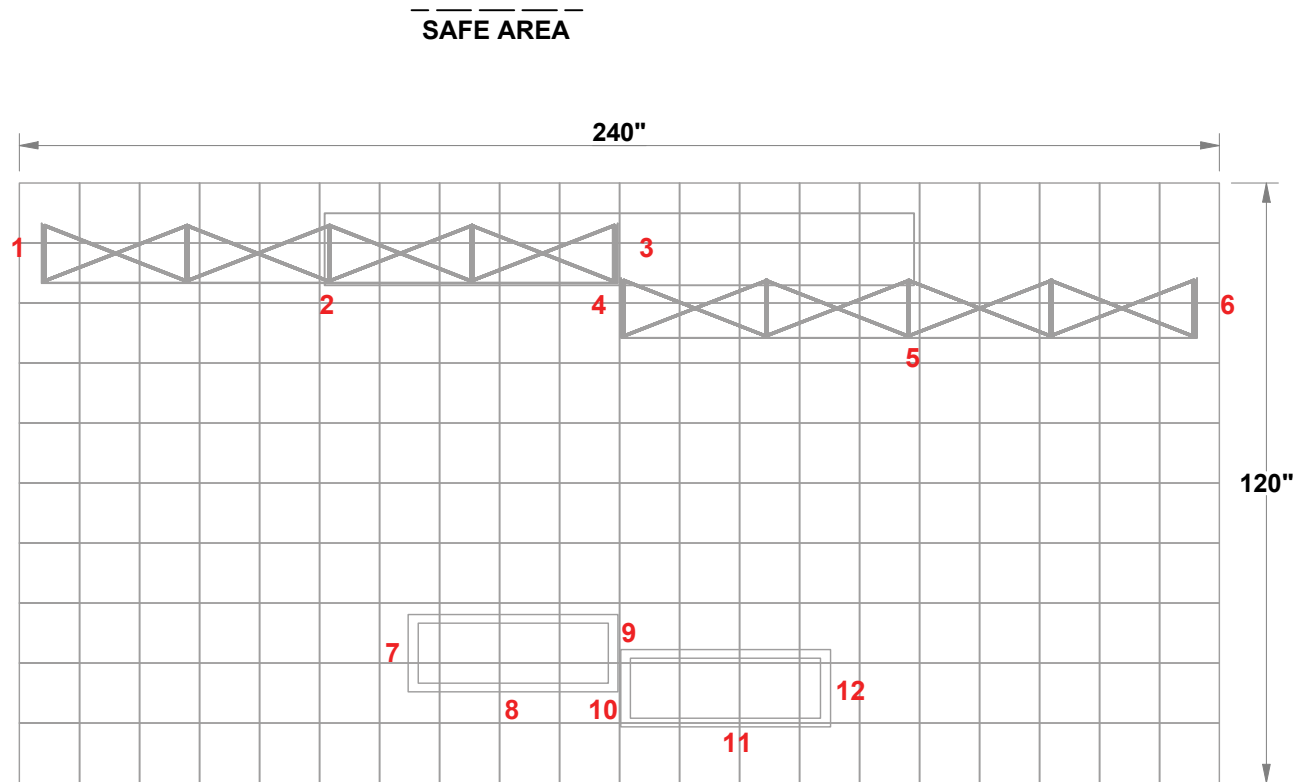
TOP VIEW
